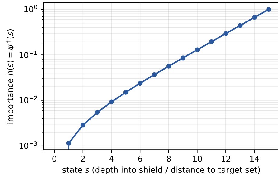
(a) Adjoint importance = committor h(s) = p h(s+1) + q h(s-1)
