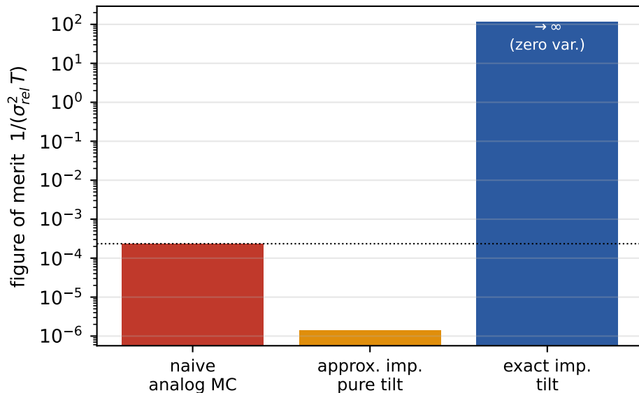
(b) Exact importance \Rightarrow zero variance; approx. pure tilt is fragile
