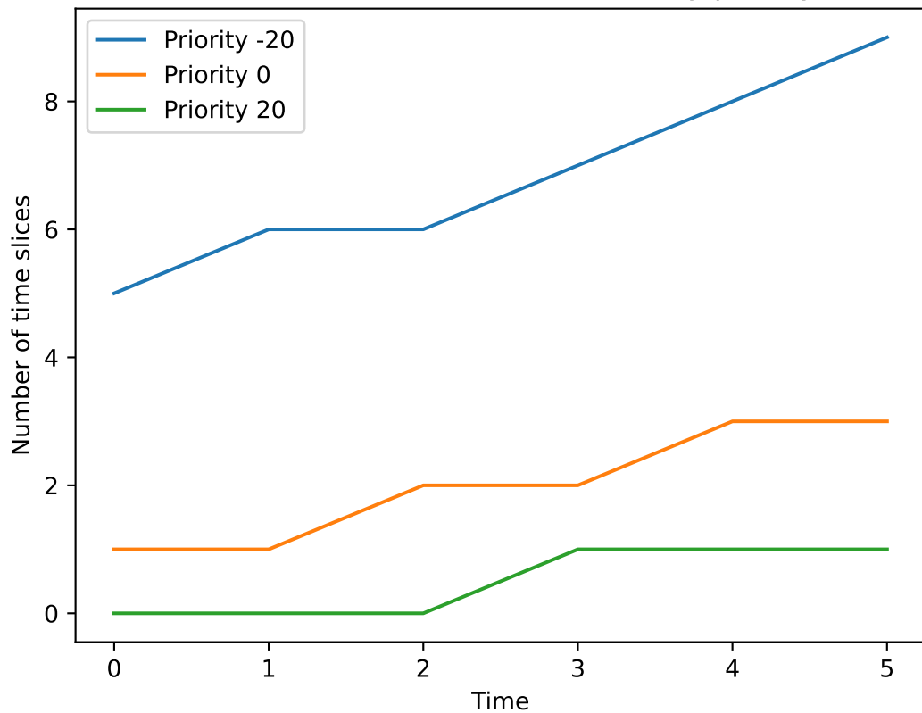
Scheduler time slices distribution by priority
