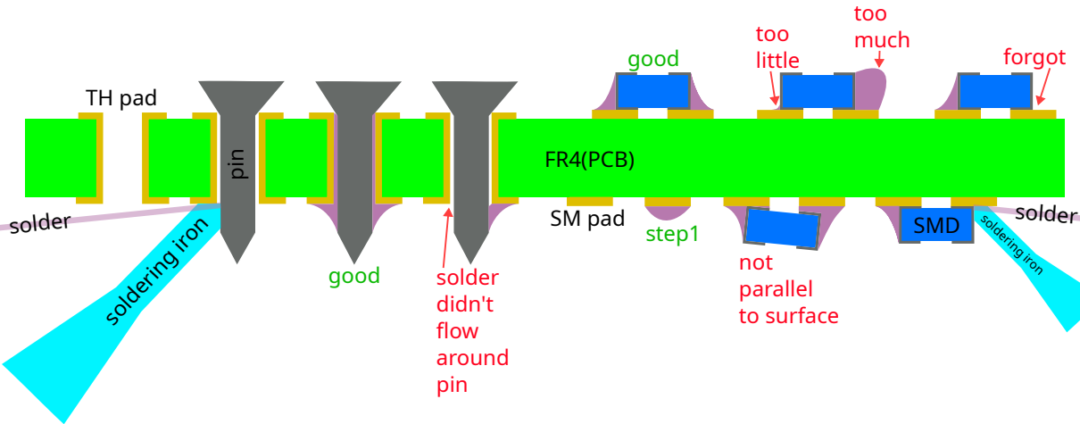
Surface-Mount Device (SMD)
