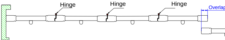
8 panels side open w/Rabbet stile
