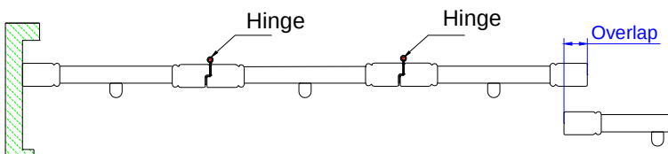
6 panels side open w/Rabbet stile
