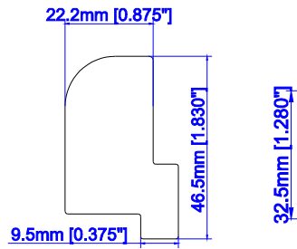
Tilt Out Z Frame
