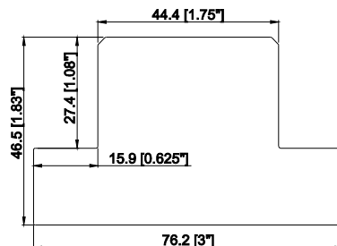
1.75" Chamfer T Post with 3/4" Light Block (L/Z/HS)
