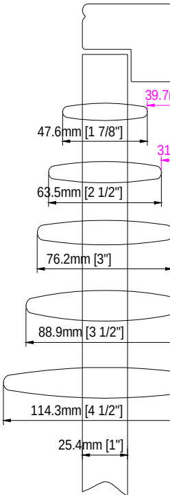
L Frame with 1" Buildout
