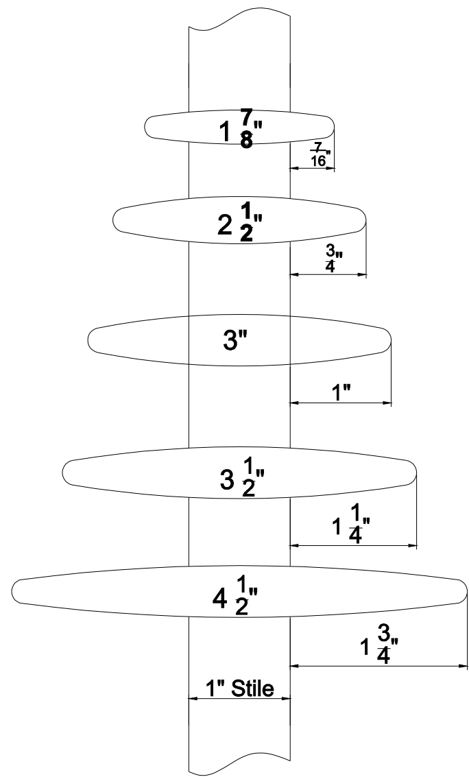
Louver Depth Clearance
