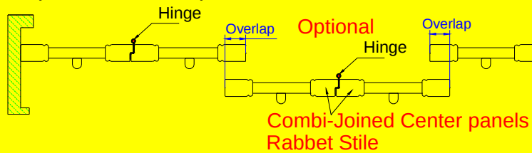
6 panels center open w/Rabbet stile
