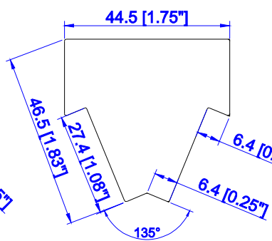
Slim Fit Bay Post for 135 Degree (L/Z/HS)
