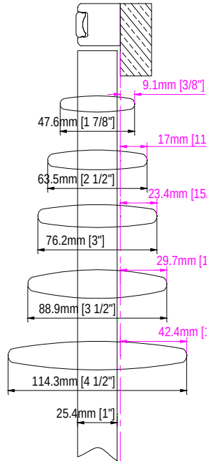
Hang Strip ( Beside the panel)
