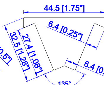
Slim Fit Bay Post for 135 Degree (L/Z/HS)
