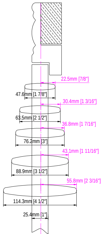
3" Crown 7 Frame
