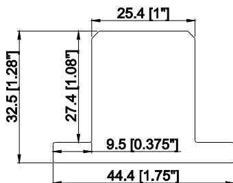
1" Chamfer T Post with 1/4" Thick x 3/8" Wide Light Block (Deco)
