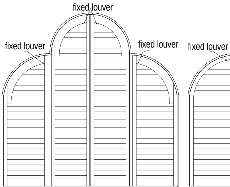
Horizontal louvers center arch with quarter round side panels -Standard louvered arch
