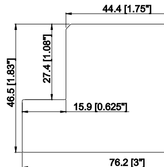
1.75" Chamfer T Post with 3/4" Light Block (L/Z/HS)
