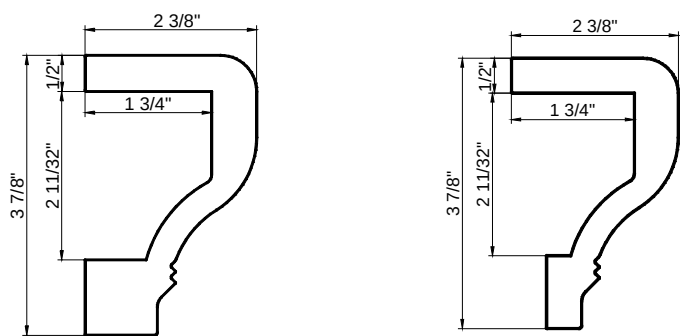
Designer Sill Cap (L)
