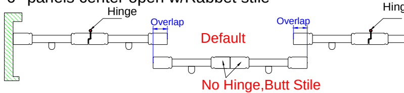
6 panels center open w/Rabbet stile
