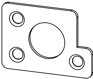
Spring loaded guide plate (for wood panel with spring loaded guide in all Bifold track)
