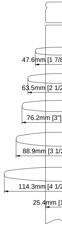
L Frame
