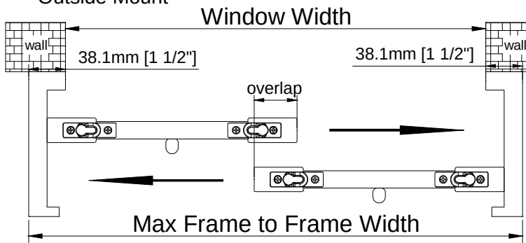
Outside Mount
