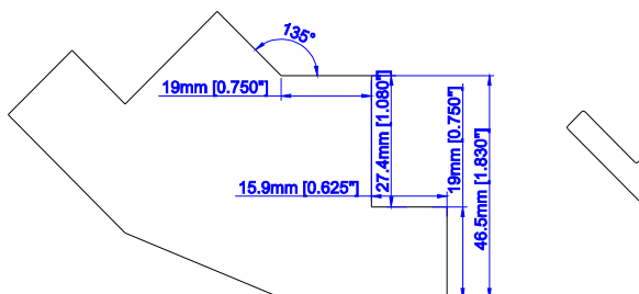
Bay Post with 3/4" Light Block (L/Z/HS)
