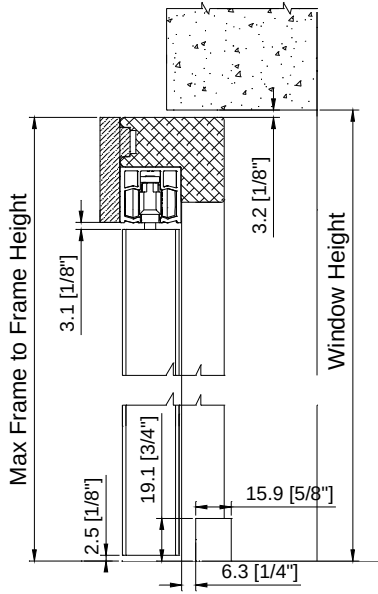
Semi-Inside
