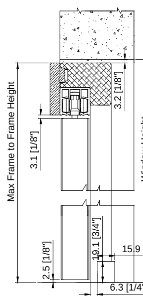
Inside Mount
