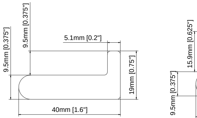
1.6" Sill Plate with 3/8" Light Block 1.6" S
