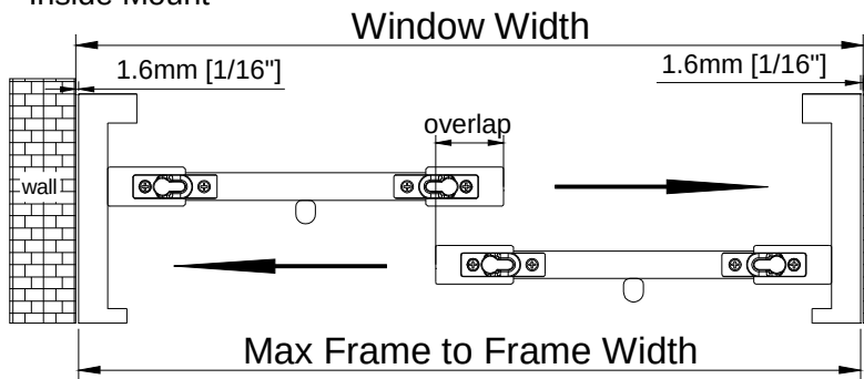
Inside Mount
