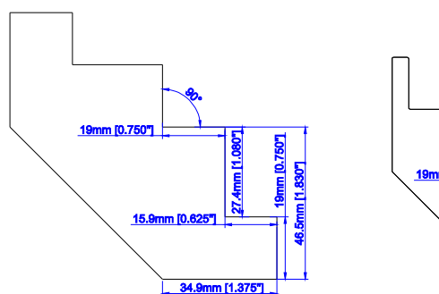
Corner Post with 3/4" Light Block (L/Z/HS)
