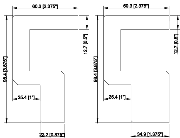
Mission Sill Cap (D/HS) Mission Sill Cap (L)
