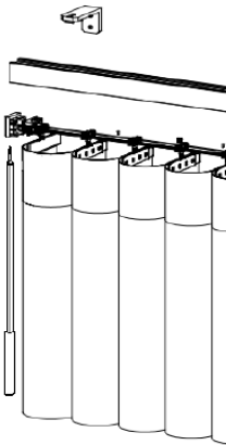
Traveling (Side by Side)
