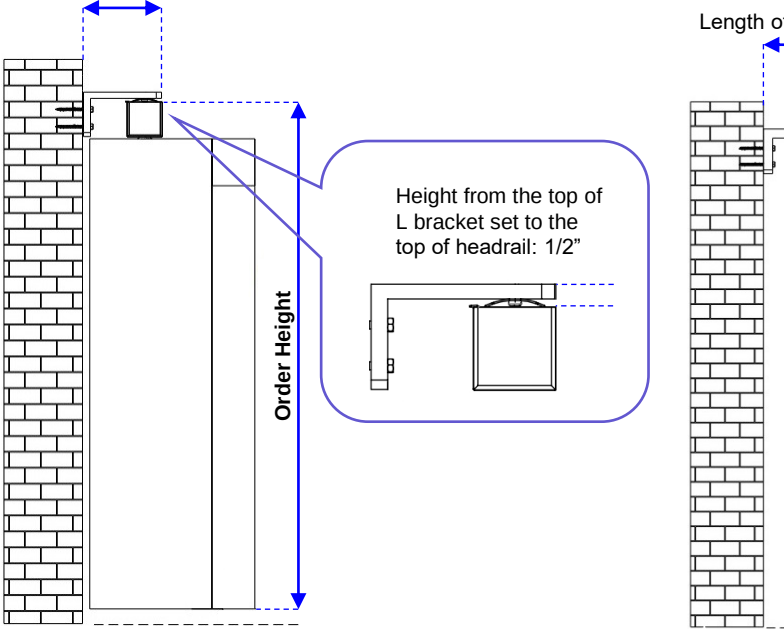
With Standard L Bracket Set
