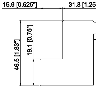
1 1/4" Beaded Z Frame
