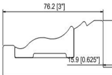
3" Ridge Deco Frame
