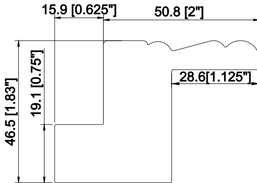
2" Belair Z Frame
