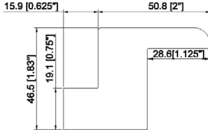
2" Bullnose Z Frame
