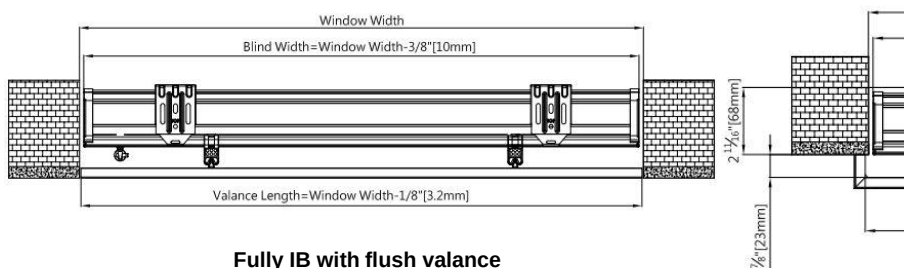
Fully IB with flush valance
