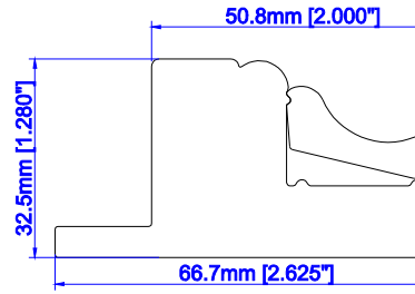
2" Classic Deco Frame
