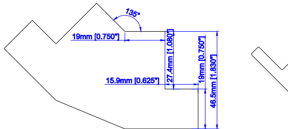
Bay Post with 3/4\" Light Block (L/Z/HS)
