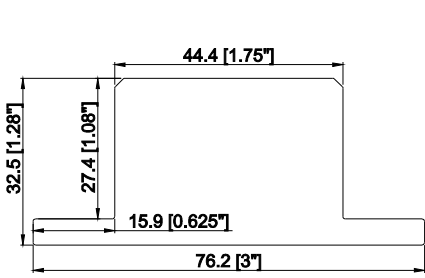
1.75" Chamfer T Post with 1/4"
