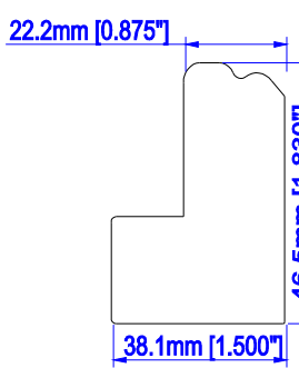
3" Crown Z Sill Plate
