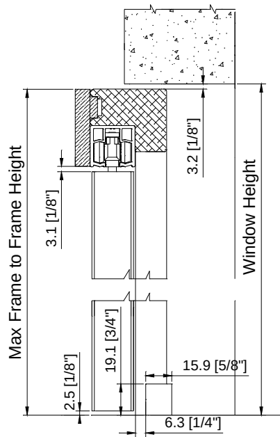
Semi-Inside
