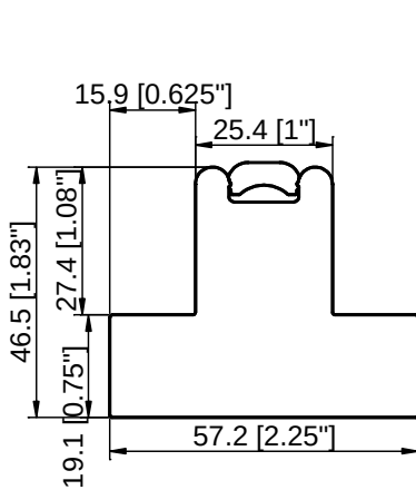
1" T Post with Insert with 3/4" Light Block
