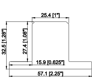
1" Chamfer T Post with 1/4" Light Block (Deco)
