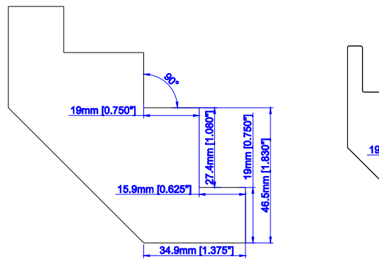
Corner Post with 3/4\" Light Block (L/Z/HS)
