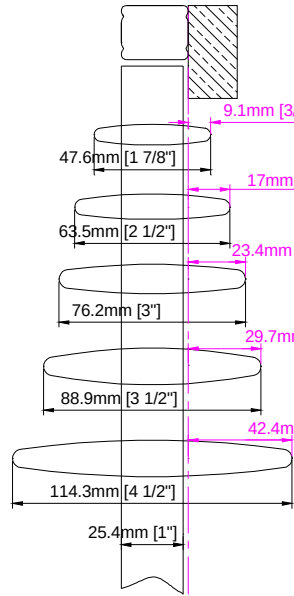
Hang Strip ( Beside the panel)
