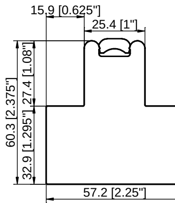
1" T Post with Insert with 1 5/16" Light Block
