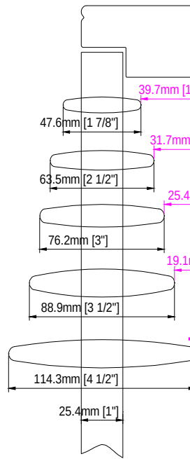
L Frame with 1" Buildout
