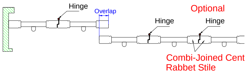
8 panels center open w/Rabbet stile
