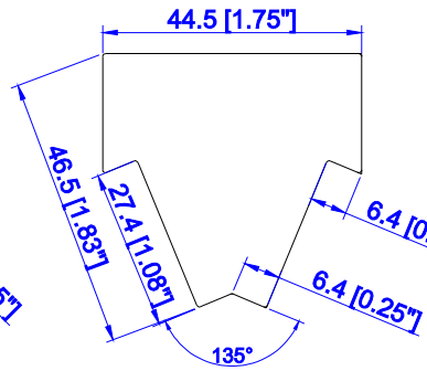
Slim Fit Bay Post for 135 Degree (L/Z/HS)
