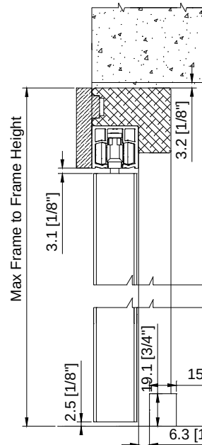
Inside Mount
