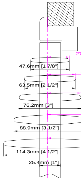
1 1/2" Bullnose Z Frame
