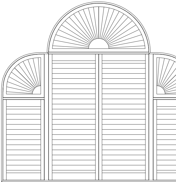
Sunburst louvers center arch with quarter round side
