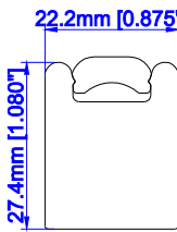
7/8" Vintage Z Not available Waterproof opt
