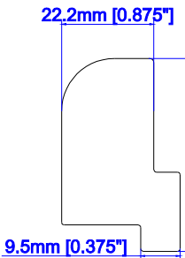
Tilt Out Z Frame
