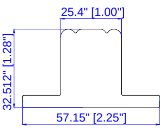
1" T Post with 1/4" Thick Light Block (Deco)
