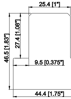
1" Chamfer T Post with 3/8" Wide Light Block (L)
