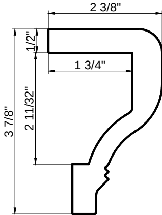
Designer Sill Cap (D/H)
