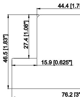
1.75" Chamfer T Post with 1/4" Light Block (L/Z/HS)
