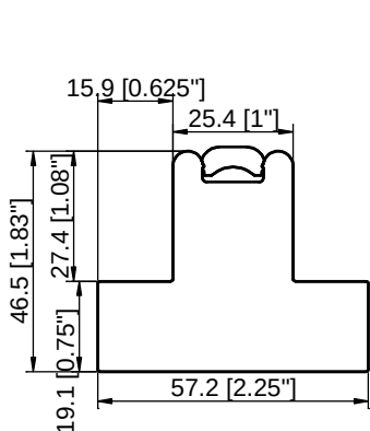
1" T Post with Insert with 3/4" Light Block
