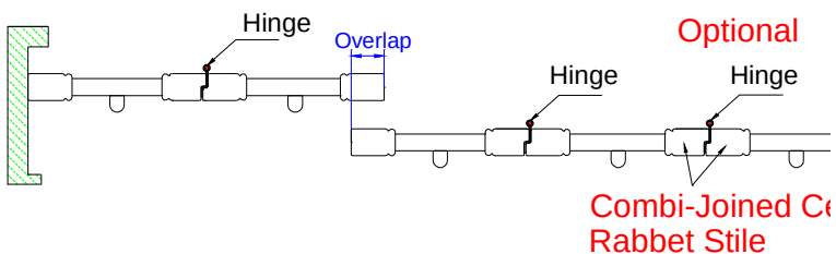
8 panels center open w/Rabbet stile
