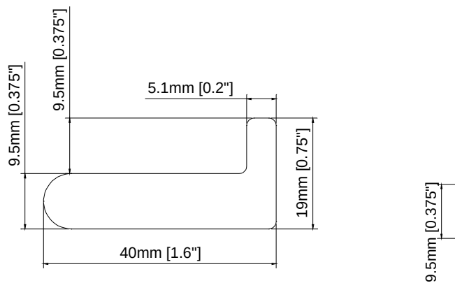
1.6" Sill Plate with 3/8" Light Block
