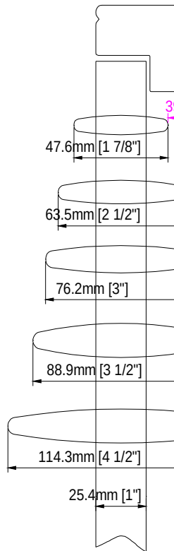
L Frame with 1" Buildout
