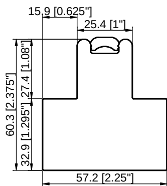
1" T Post with Insert with 1 5/16" Light Block
