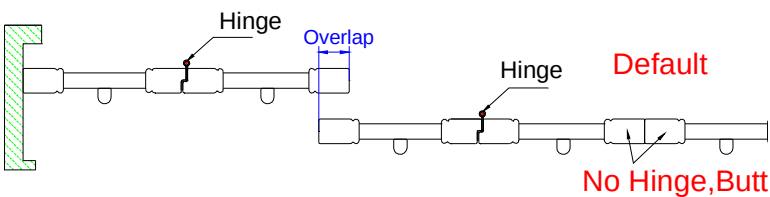
8 panels center open w/Rabbet stile
