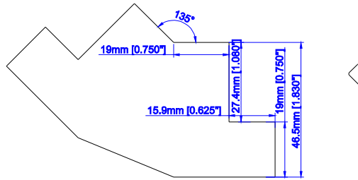
Bay Post with 3/4" Light Block (L/Z/HS)
