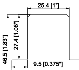
1" T Post with Insert with 1 5/16" Light Block
