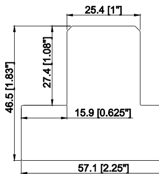
1" Chamfer T Post with 1/4" Light Block (L/Z/HS)
