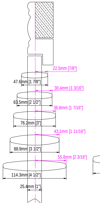
3" Crown Z Frame
