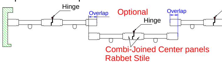
6 panels center open w/Rabbet stile
