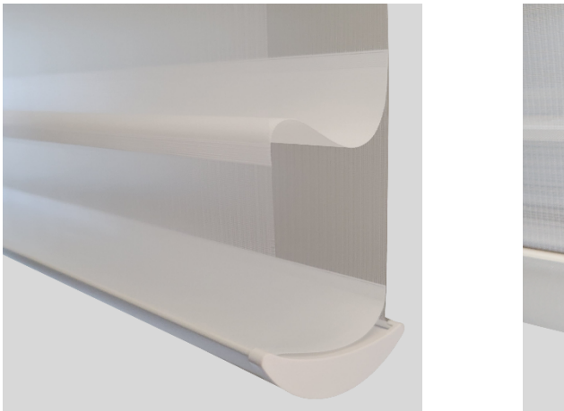
<Moon Shape>
