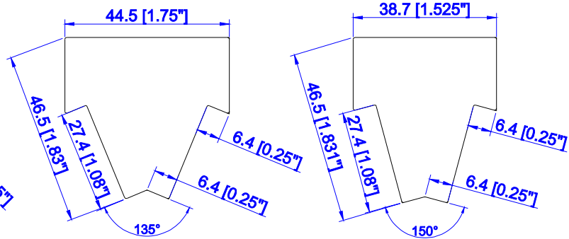
Slim Fit Bay Post for 135 Degree (L/Z/HS)
