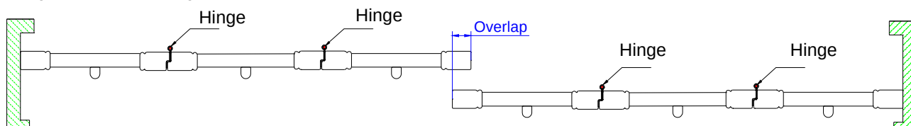
6 panels side open w/Rabbit stile
