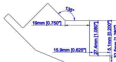
Bay Post with 1/4" Light Block (Deco)
