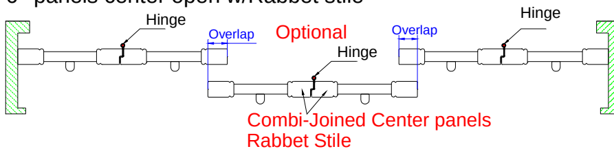
6 panels center open w/Rabbet stile
