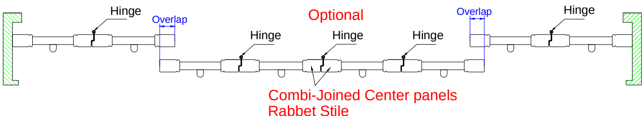
8 panels center open w/Rabbet stile
