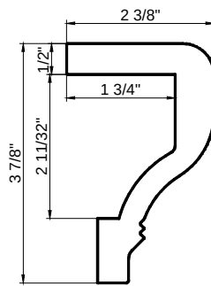
Designer Sill Cap (D/HS)
