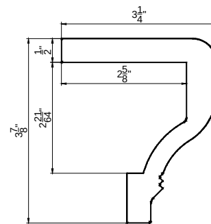
Designer Sill Cap (Z)
