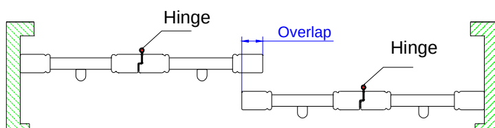
4 panels side open w/Rabbit stile
