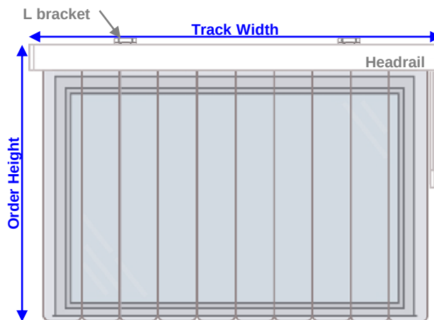
Wall Mount
