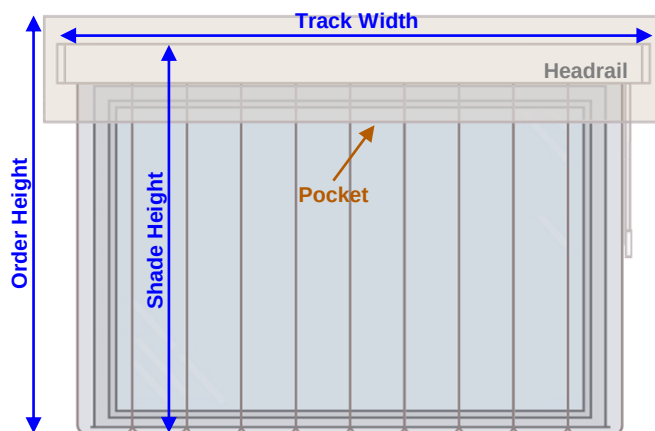
Ceiling Pocket Mount
