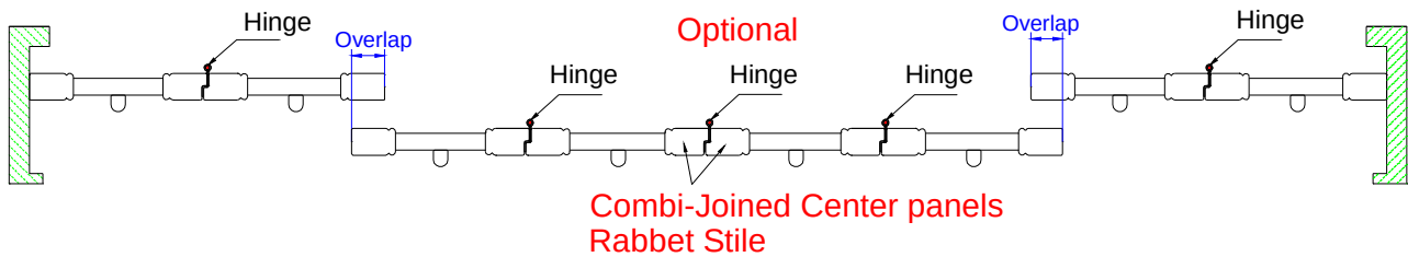
8 panels center open w/Rabbet stile
