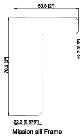
Mission sill Frame
