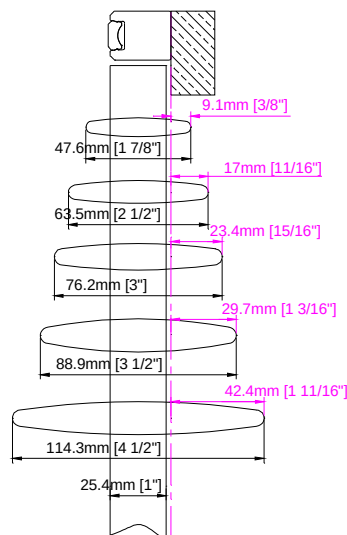
Hang Strip ( Beside the panel)
