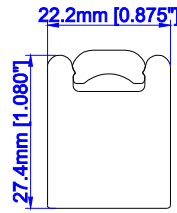
7/8" Vintage Hang Strip Not available for Waterproof option
