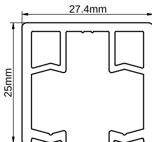
Top Track
