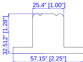
1" T Post with 1/4" Thick Light Block (Deco)
