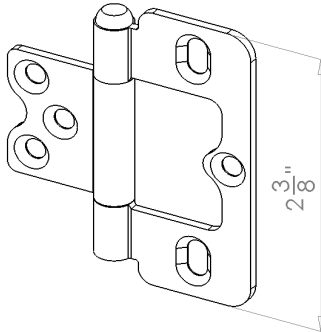
2.375" Self-Mortise Hinge
