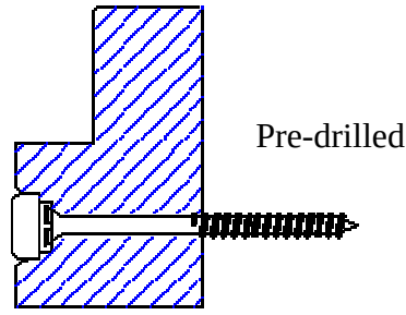
Deep Plain L frame
