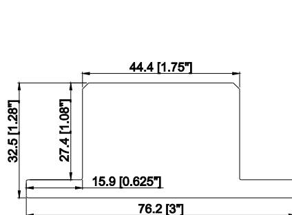
1.75" Chamfer T Post with 1/4" Light Block (Deco)
