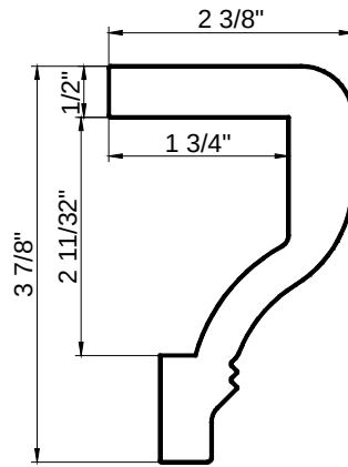
Designer Sill Cap (D/HS)
