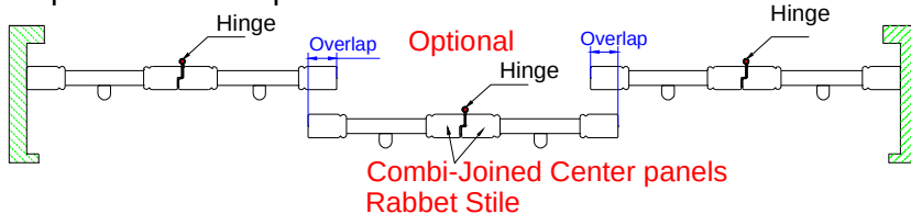
6 panels center open w/Rabbet stile
