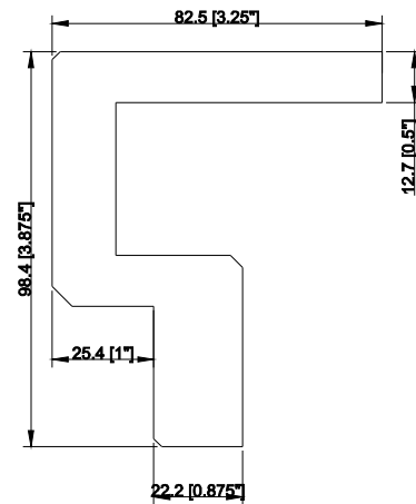
Mission Sill Cap (Z)
