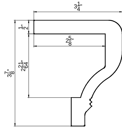
Designer Sill Cap (Z)
