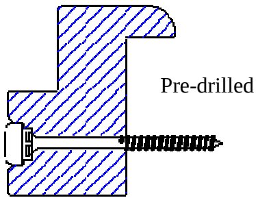
1 1/2" Deep Bullnose Z frame
