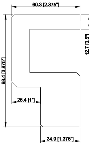
Mission Sill Cap (L)
