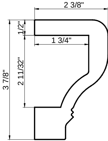
Designer Sill Cap (L)
