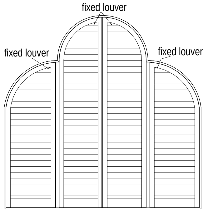
Horizontal louvers center arch with quarter round side panels -Continuous arch Not available for Waterproof option.
