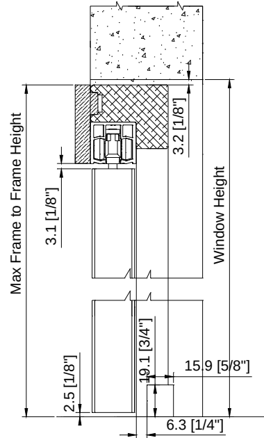
Inside Mount
