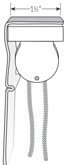
CLUTCH SHADE
