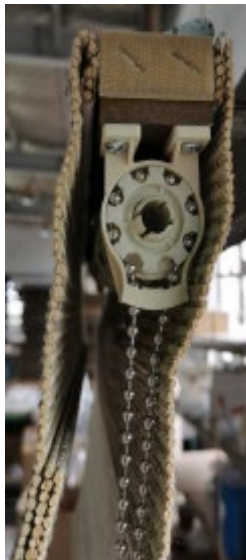
Slim clutch with 1.5" headrail for a narrower mounting installation.
