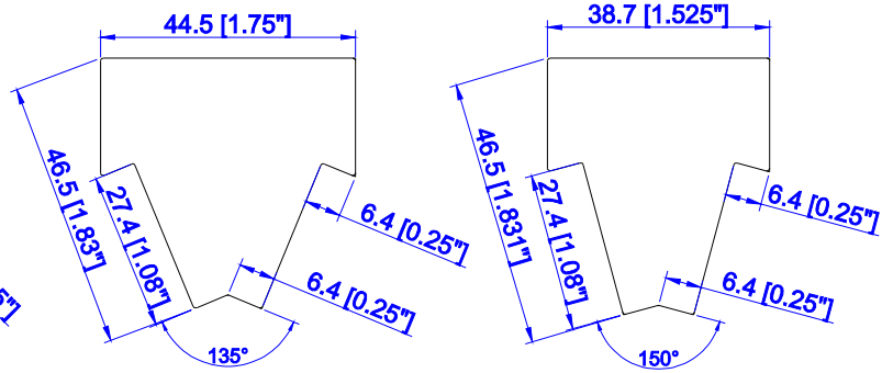
Slim Fit Bay Post for 135 Degree (L/Z/HS)
