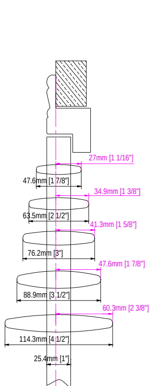
2" Bel Air Z Frame
