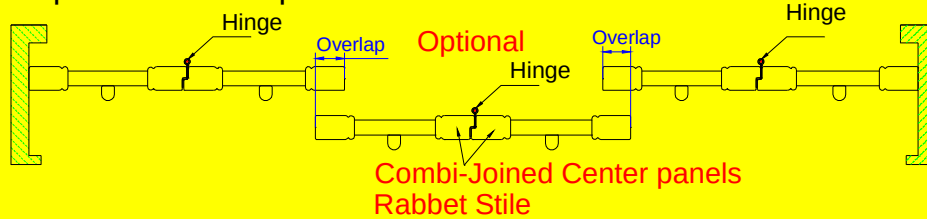
6 panels center open w/Rabbet stile
