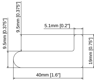
1.6" Sill Plate with 3/8" Light Block
