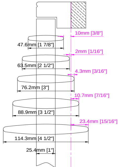
L Frame
