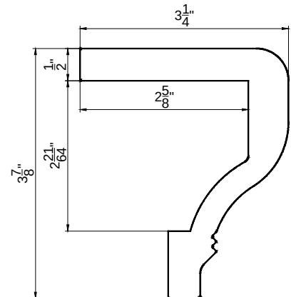
Designer Sill Cap (Z)
