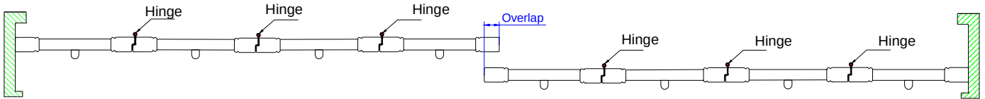
8 panels side open w/Rabbet stile
