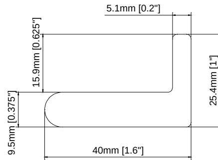
1.6" Sill Plate with 5/8" Light Block
