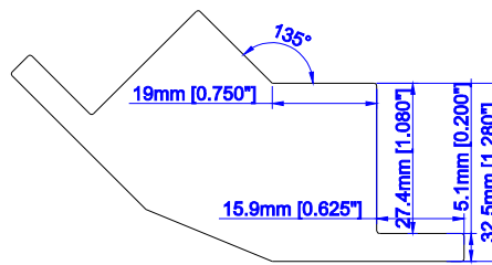
Bay Post with 1/4" Light Block (Deco)
