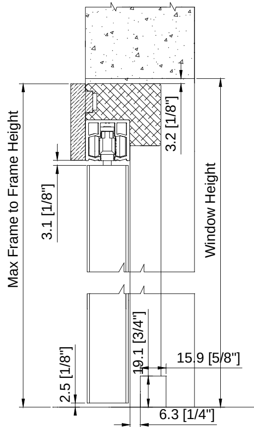
Inside Mount
