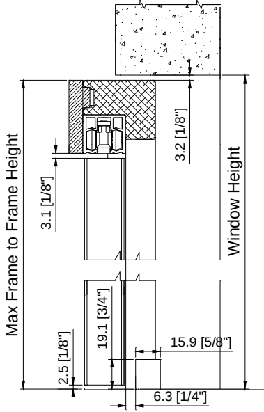
Semi-Inside
