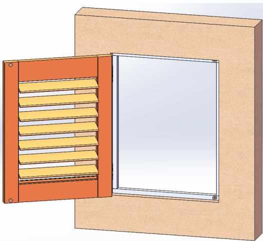
Light block
