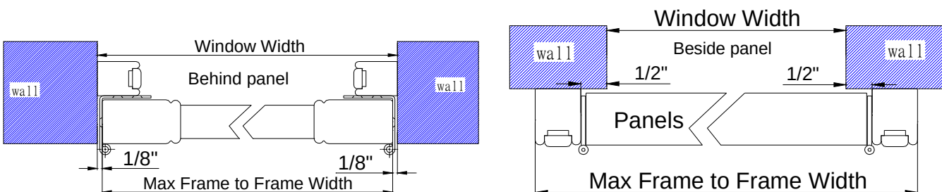
Quarter Round
