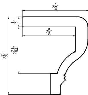
Designer Sill Cap (Z)
