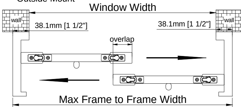
Outside Mount
