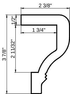
Designer Sill Cap (D/HS)
