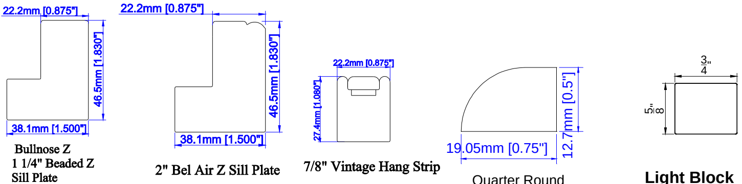
Quarter Round
