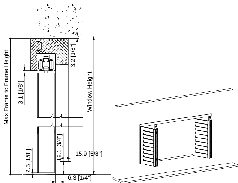
Inside Mount
