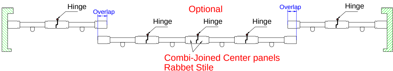
8 panels center open w/Rabbit stile
