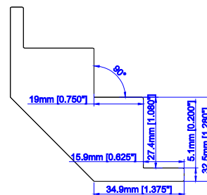
Corner Post with 1/4" Light Block (Deco)
