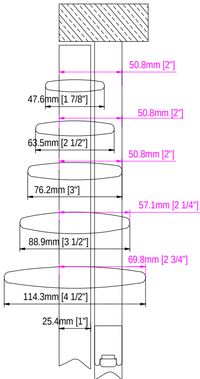
Hang Strip ( Behind the panel)
