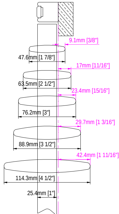
Hang Strip ( Beside the panel)
