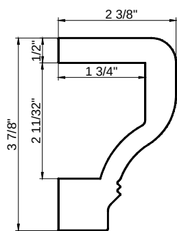
Designer Sill Cap (L)
