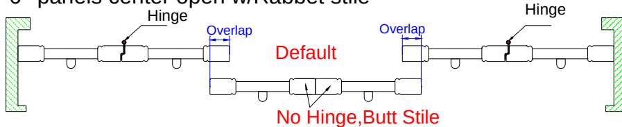
6 panels center open w/Rabbit stile
