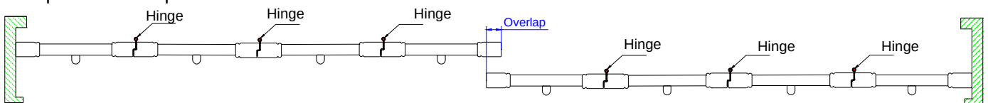
8 panels side open w/Rabbit stile
