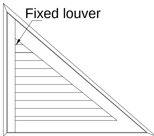
Right Triangle
