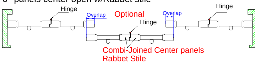
6 panels center open w/Rabbit stile
