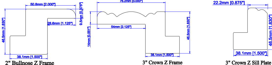
2" Bullnose Z Frame
