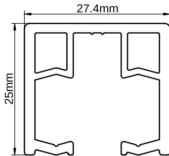
Top Track
