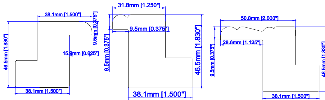
1 1/2" Bullnose Z Frame
