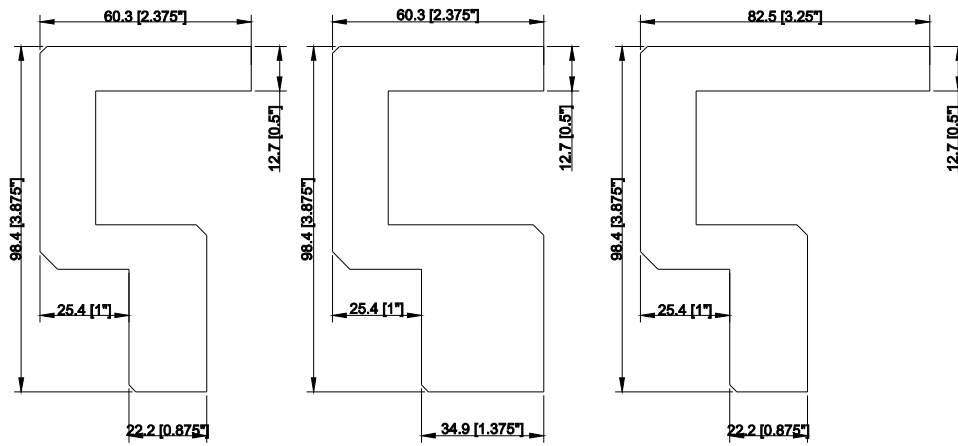
Mission Sill Cap (D/HS)
