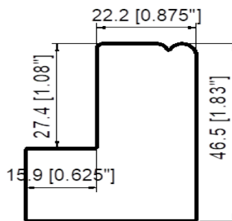
Beaded L frame
