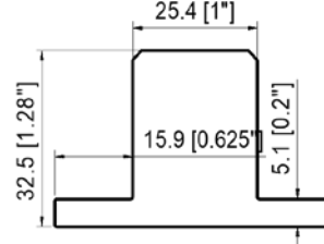
(Optional T Post)
