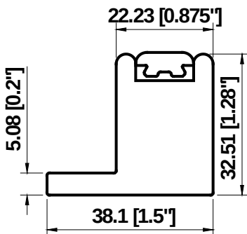
Vintage L Frame with Insert (1/4" Light Block)
