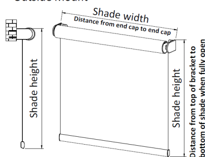
Outside Mount
