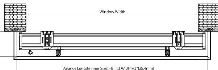
OB with Valance and returns
