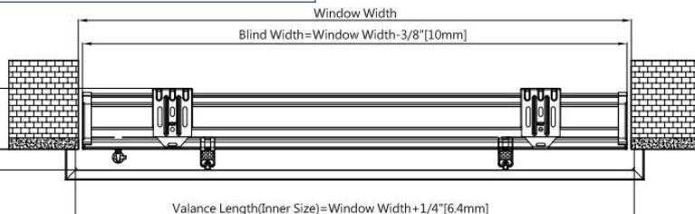
Semi-IB with bracket flush to wall
