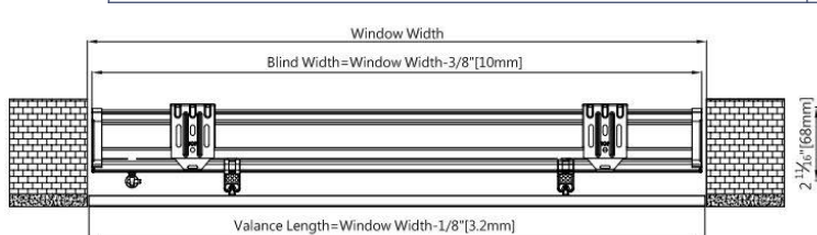
Fully IB with flush valance
