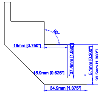
Corner Post with 1/4" Light Block (Deco)
