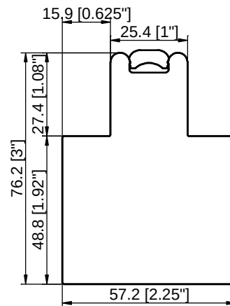
1" T Post with Insert with 1 15/16" Light Block
