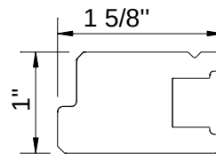
1 5/8" Rabbet Stile-R
