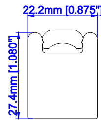
7/8" Vintage Hang Strip
