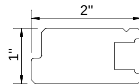
2" Rabbet Stile-R
