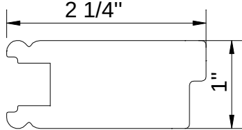
2 1/4" Rabbet Stile
