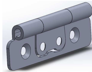
2.375" Bi-fold Hinge
