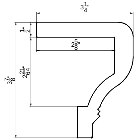
Designer Sill Cap (Z)
