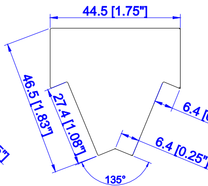
Slim Fit Bay Post for 135 Degree (L/Z/HS)
