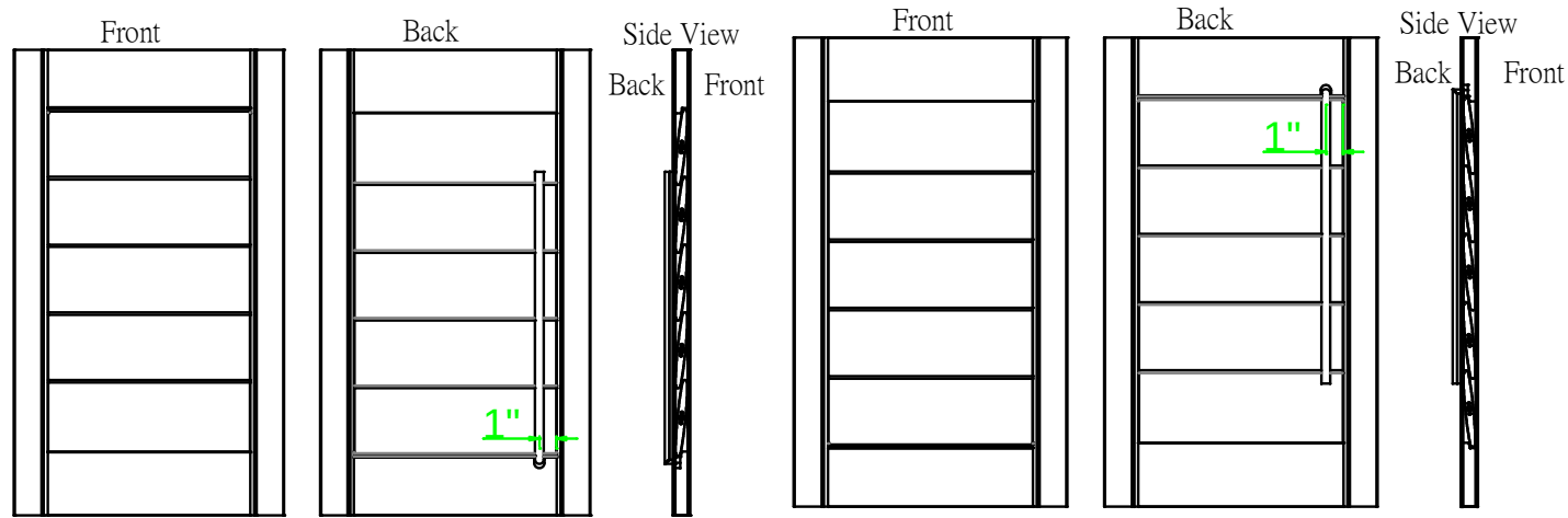
Offset tilt rod on the back side of panel, the louvers dress up from front view
