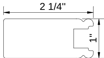
2 1/4" Butt Stile
