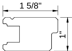
1 5/8" Rabbet Stile-L
