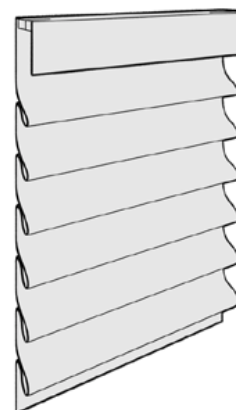
Hobbled Shade Mins W- 18" H- 24" Max W- 96" H- 96" 6" Front Valance
