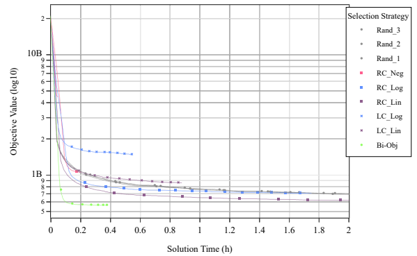
Figure 1: The LP objective value (on a \log_{10} scale) plotted against the wall-clock hours for various selection strategies (configuration: Pool_Selection). Each marker represents every 10 column generation iteration.
