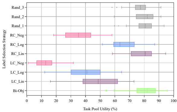
Figure 9: The spread of each employee's task pool utility for different label selection strategies (configuration: Pool_Selection). Utility is the number of unique tasks in negative reduced cost columns generated by an employee as a percentage of the total number of unique tasks in an employee's task pool. Note that for the unrestricted-task pools, each employee's task pool contains every task in the employee's eligible task set.
