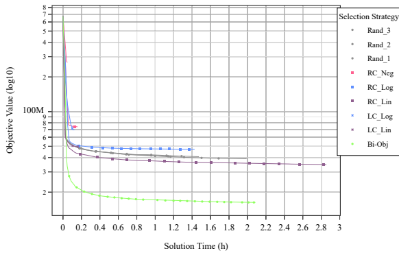
Figure 1: The LP objective value (on a \log_{10} scale) plotted against the wall-clock hours for various selection strategies (configuration: Pool_Selection). Each marker represents every 10 column generation iteration.
