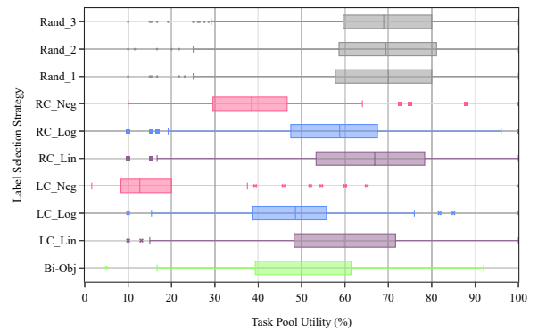
Figure 9: The spread of each employee's task pool utility for different label selection strategies (configuration: Pool_Selection). Utility is the number of unique tasks in negative reduced cost columns generated by an employee as a percentage of the total number of unique tasks in an employee's task pool. Note that for the unrestricted-task pools, each employee's task pool contains every task in the employee's eligible task set.
