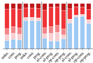
Gemini 2.5
