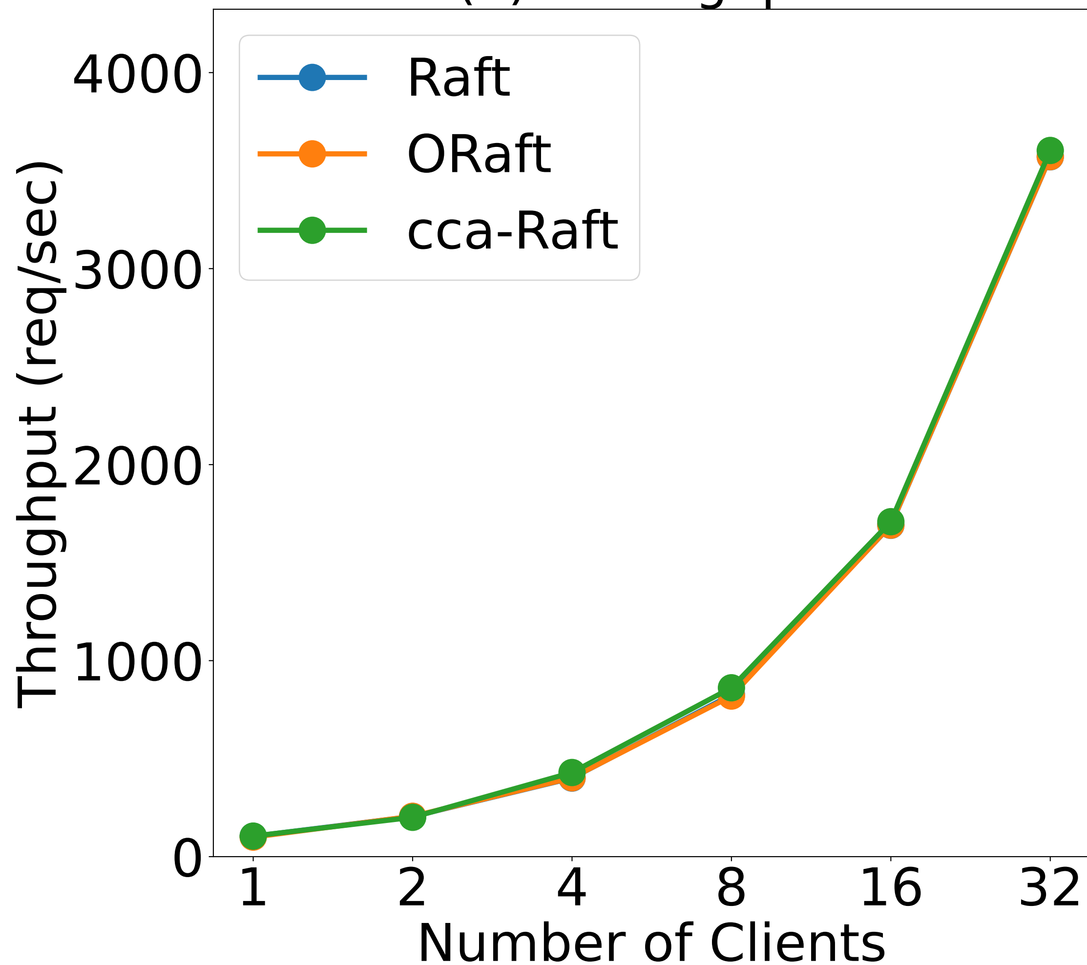
(a) Throughput
