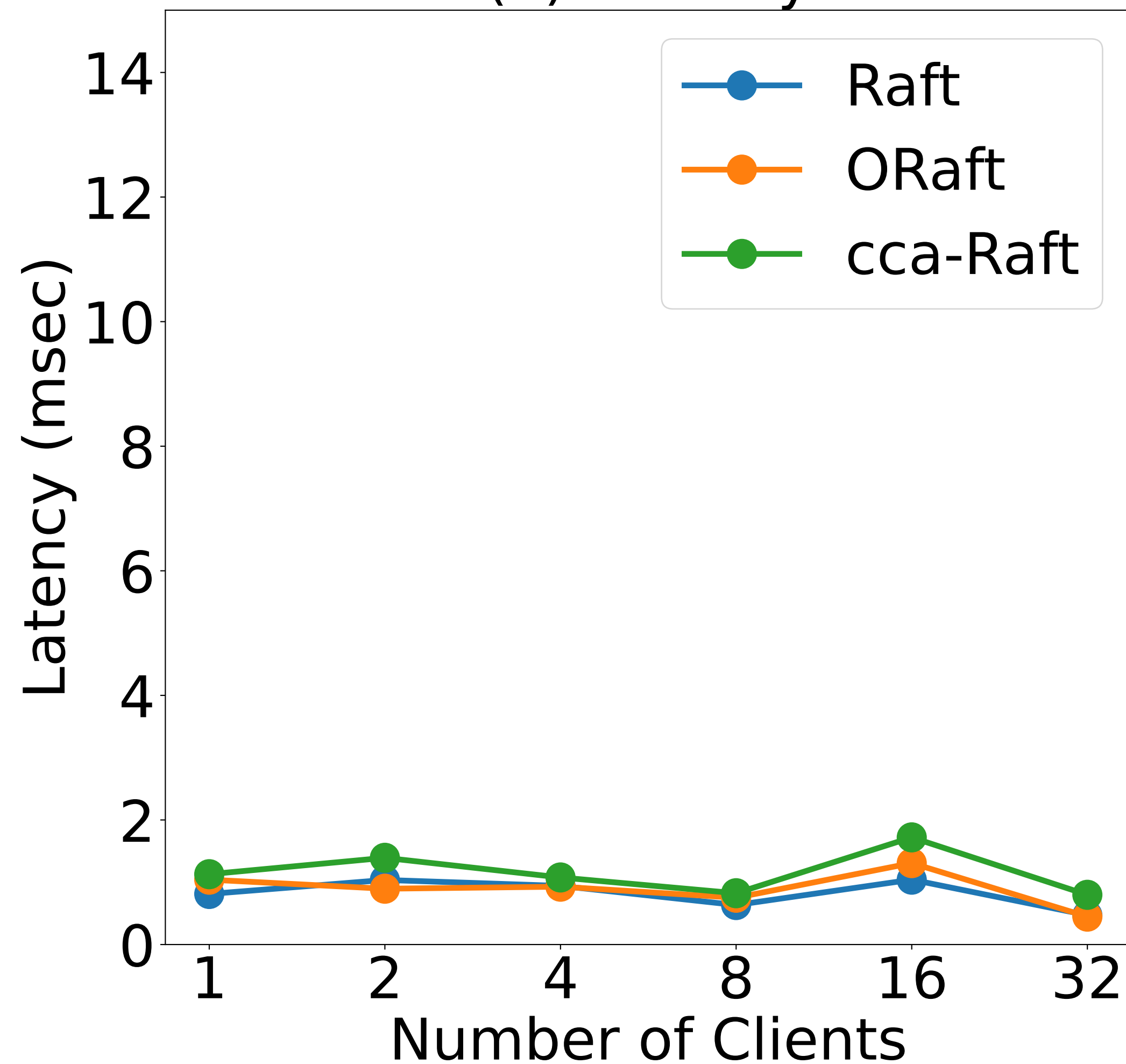
(b) Latency
