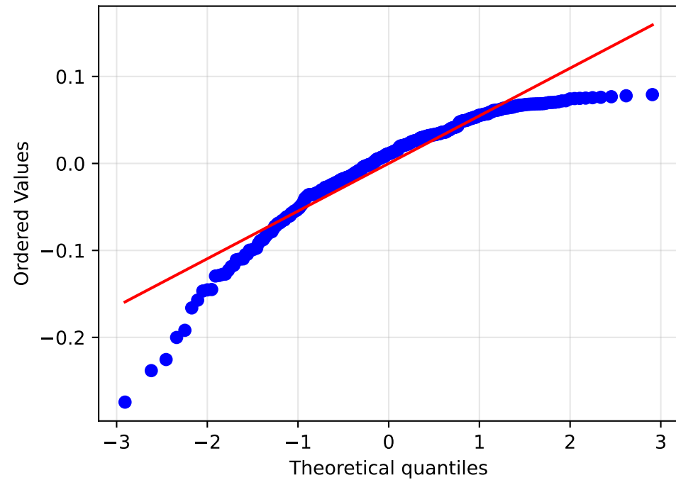
Q-Q Plot: Dice coefficient
