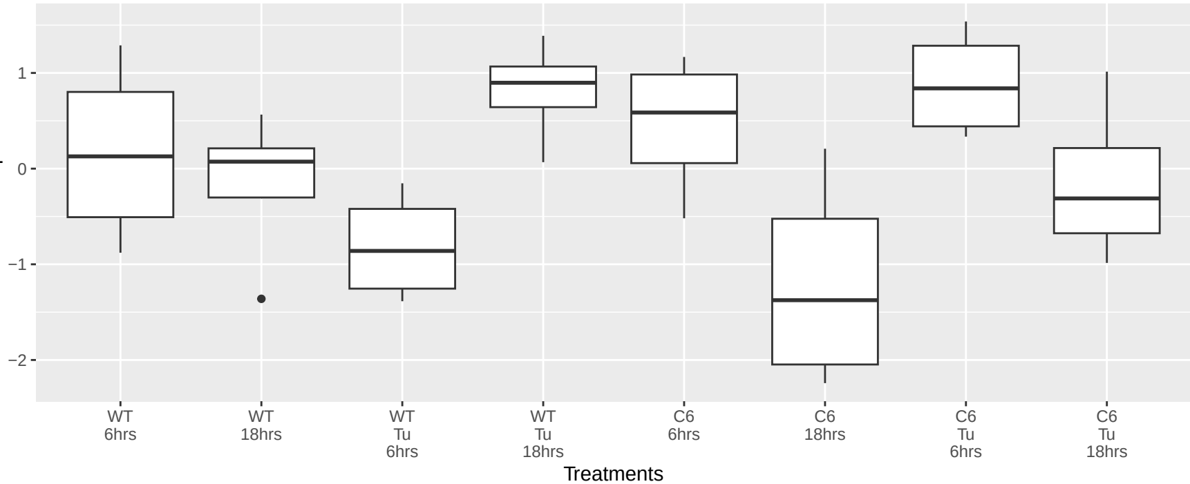
ELF1.P32519 Expression
