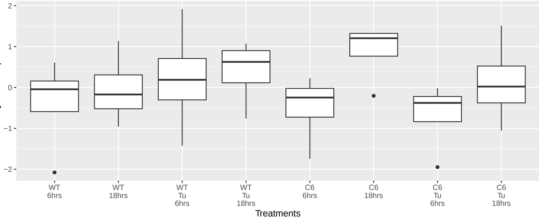
EXOSC8.Q96B26 Expression
