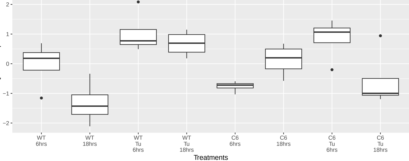
HSPH1.Q92598 Expression
