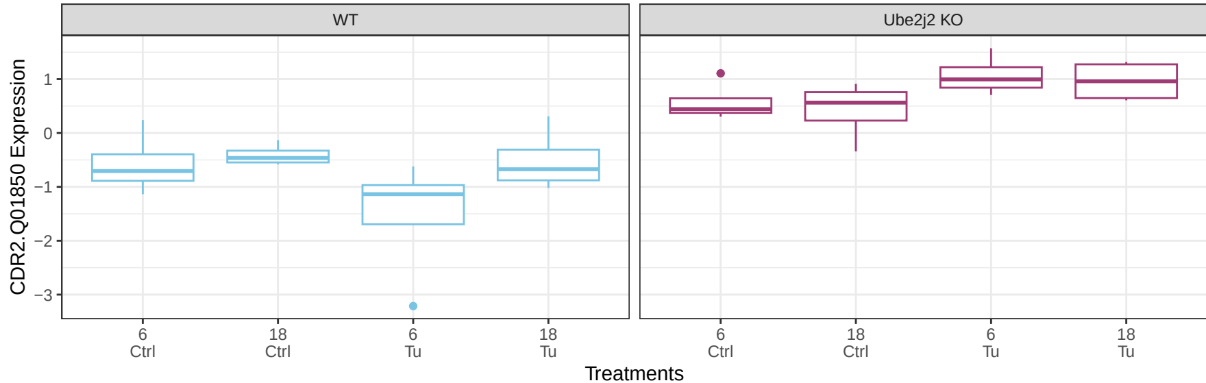
CDR2.Q01850 occurs in the magenta module
