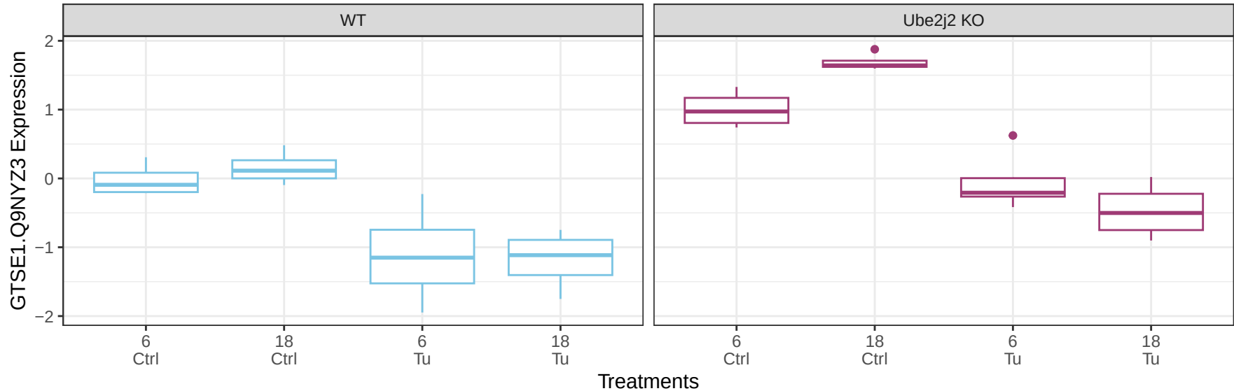
GTSE1.Q9NYZ3 occurs in the cyan module
