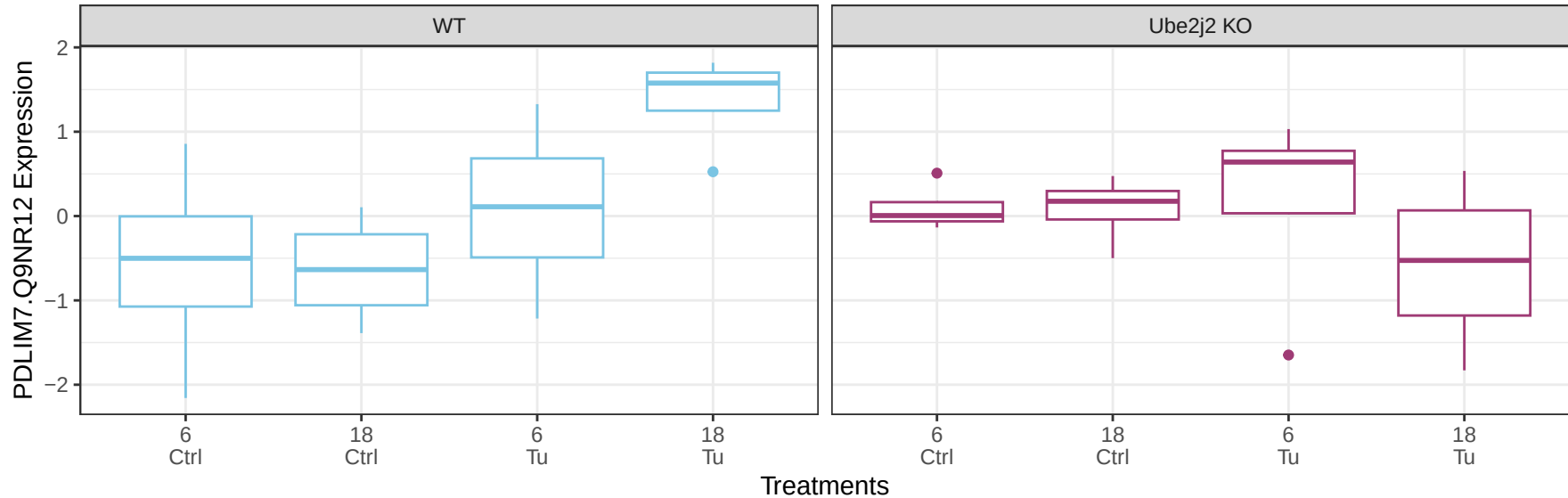
PDLIM7.Q9NR12 occurs in the black module
