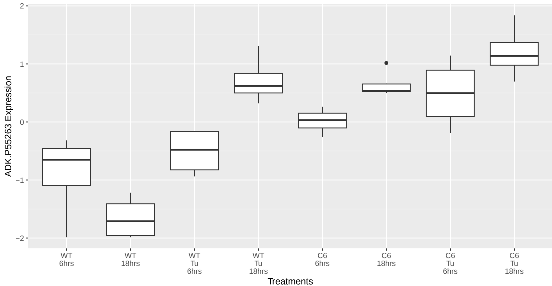
ADK.P55263 occurs in the blue module
