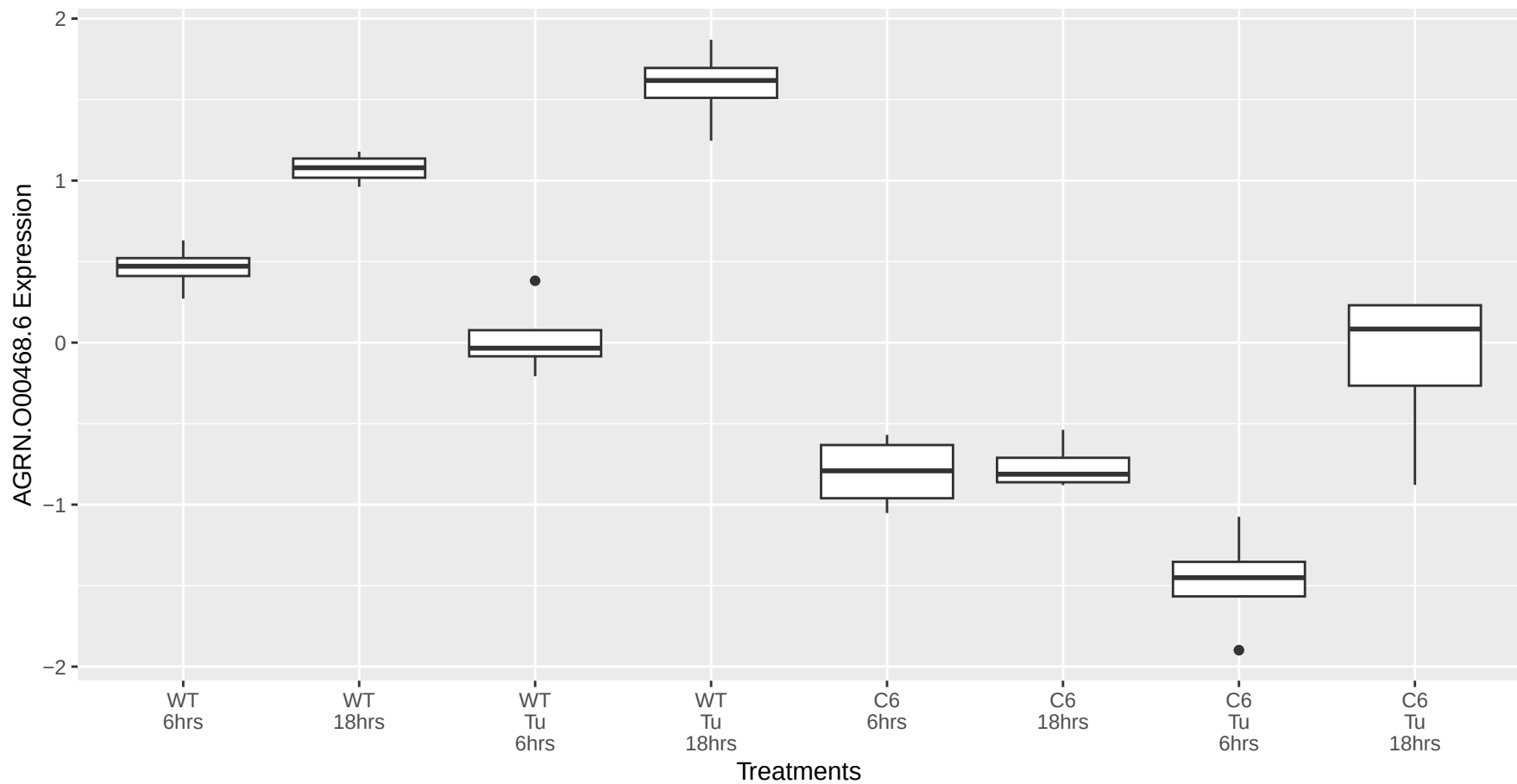
AGRN.O00468.6 occurs in the salmon module
