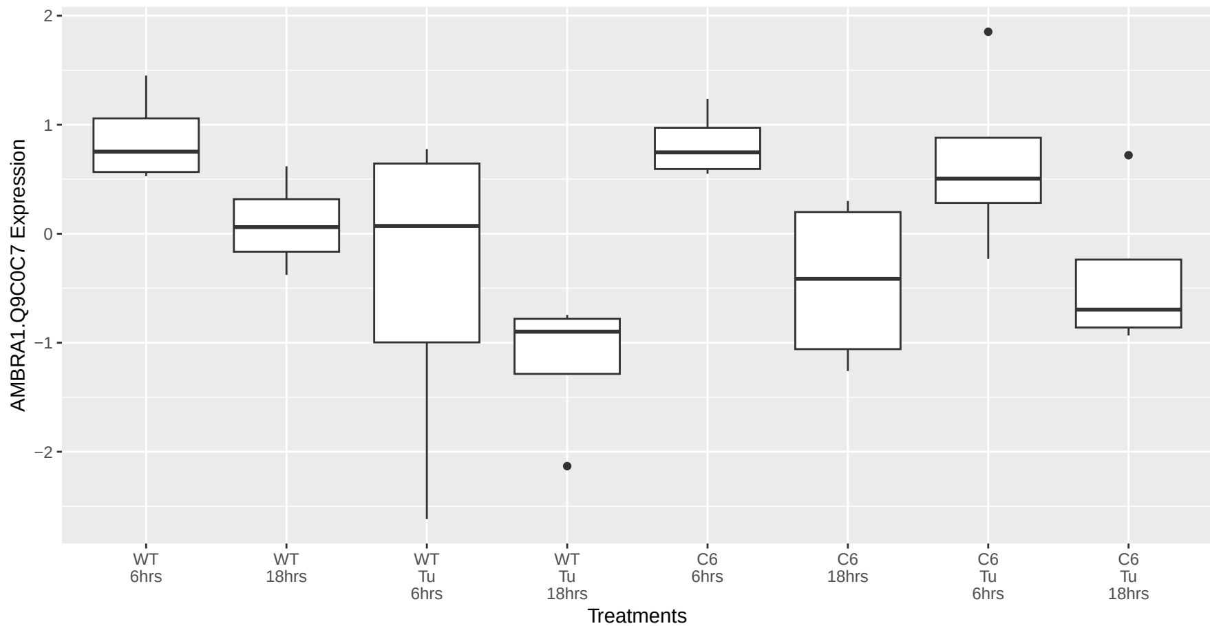
AMBRA1.Q9C0C7 occurs in the yellow module
