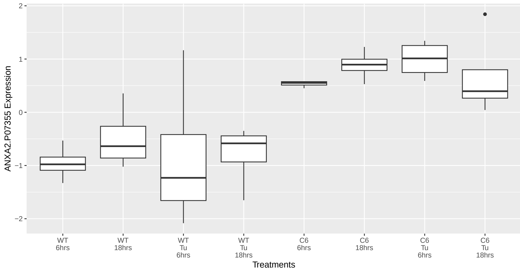
ANXA2.P07355 occurs in the magenta module
