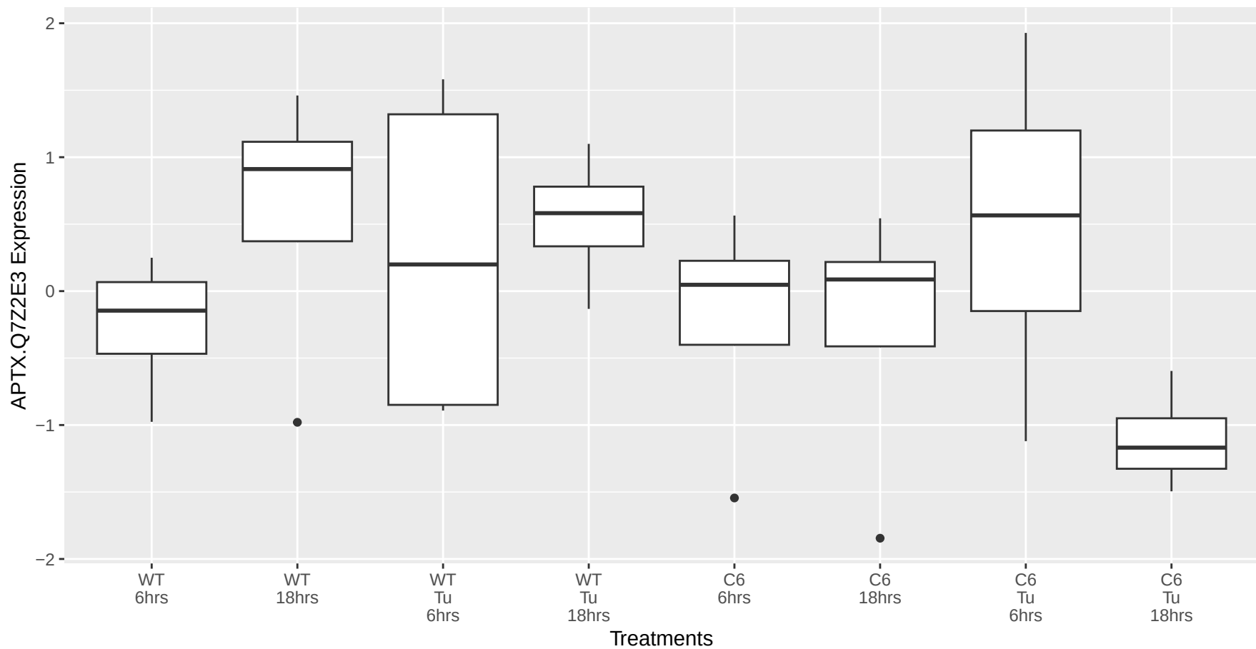
APTX.Q7Z2E3 occurs in the brown module
