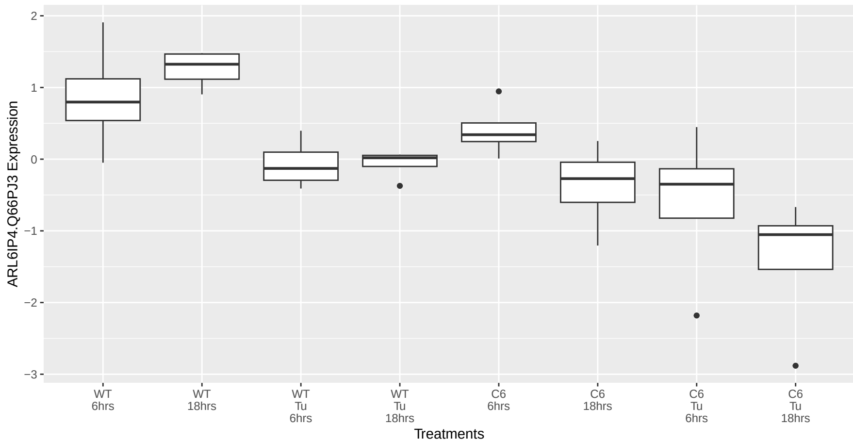
ARL6IP4.Q66PJ3 occurs in the blue module
