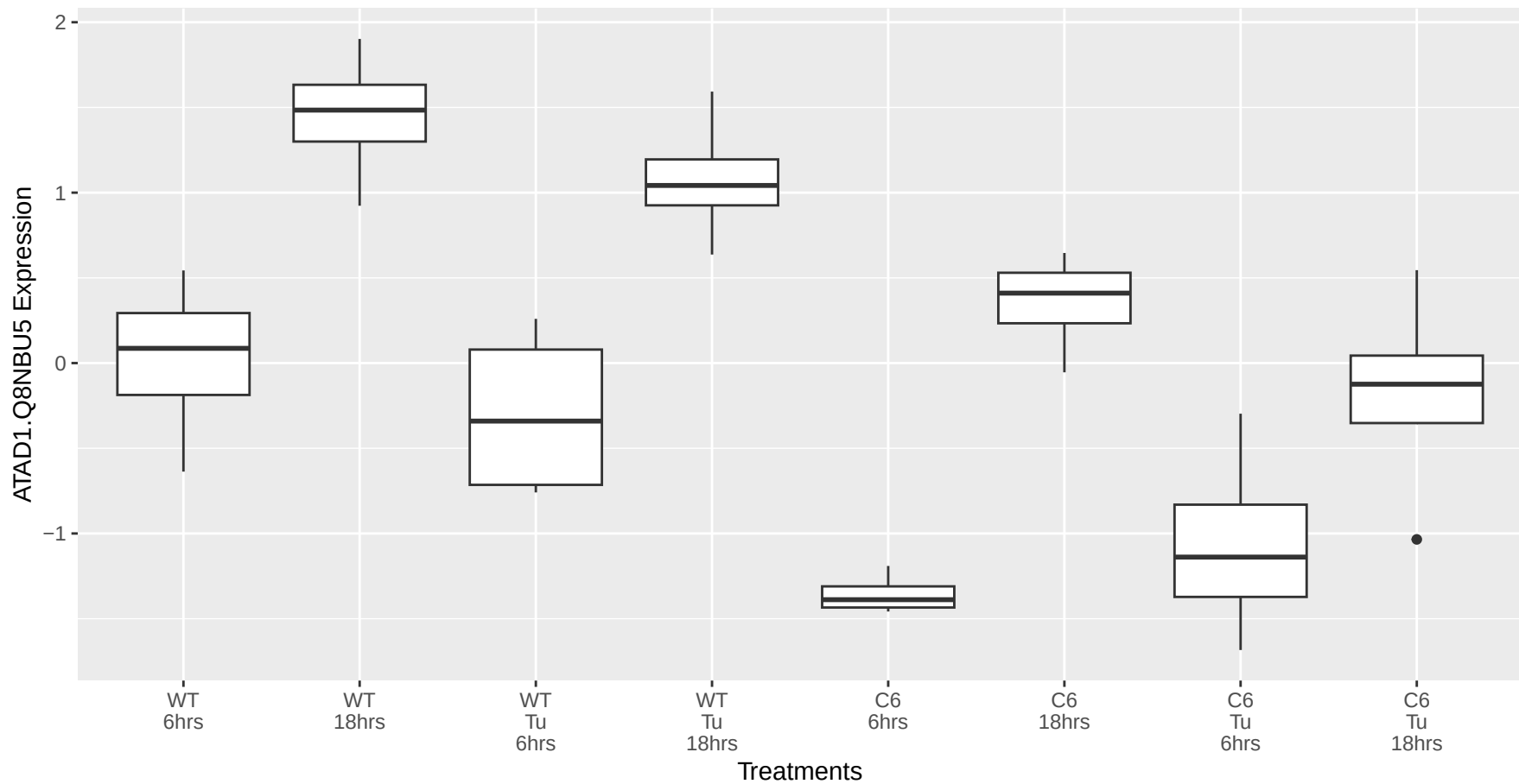
ATAD1.Q8NBU5 occurs in the salmon module
