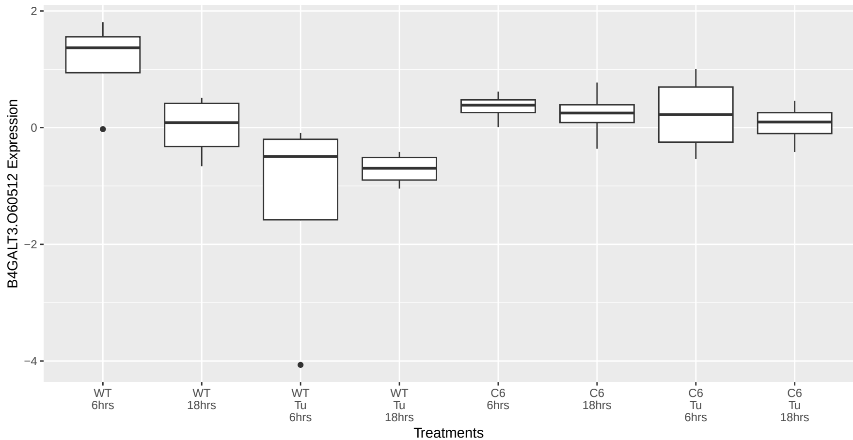
B4GALT3.O60512 occurs in the black module
