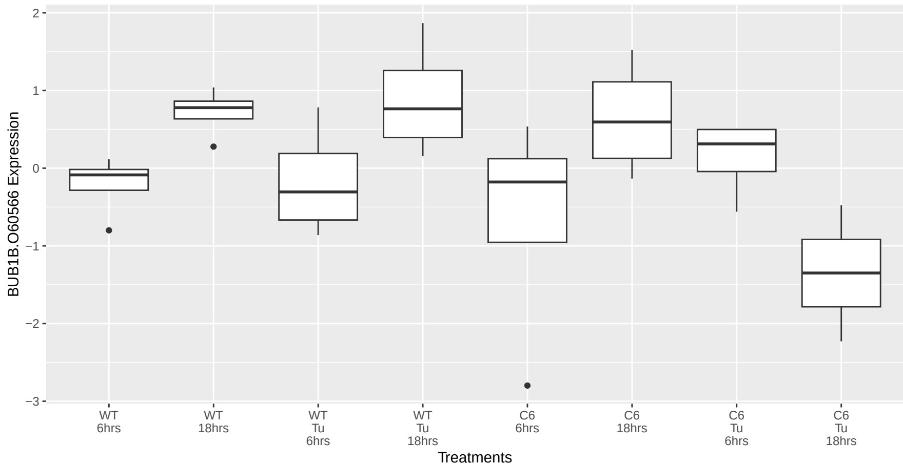
BUB1B.O60566 occurs in the brown module
