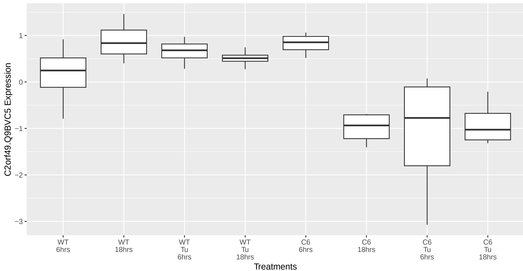
C2orf49.Q9BVC5 occurs in the magenta module
