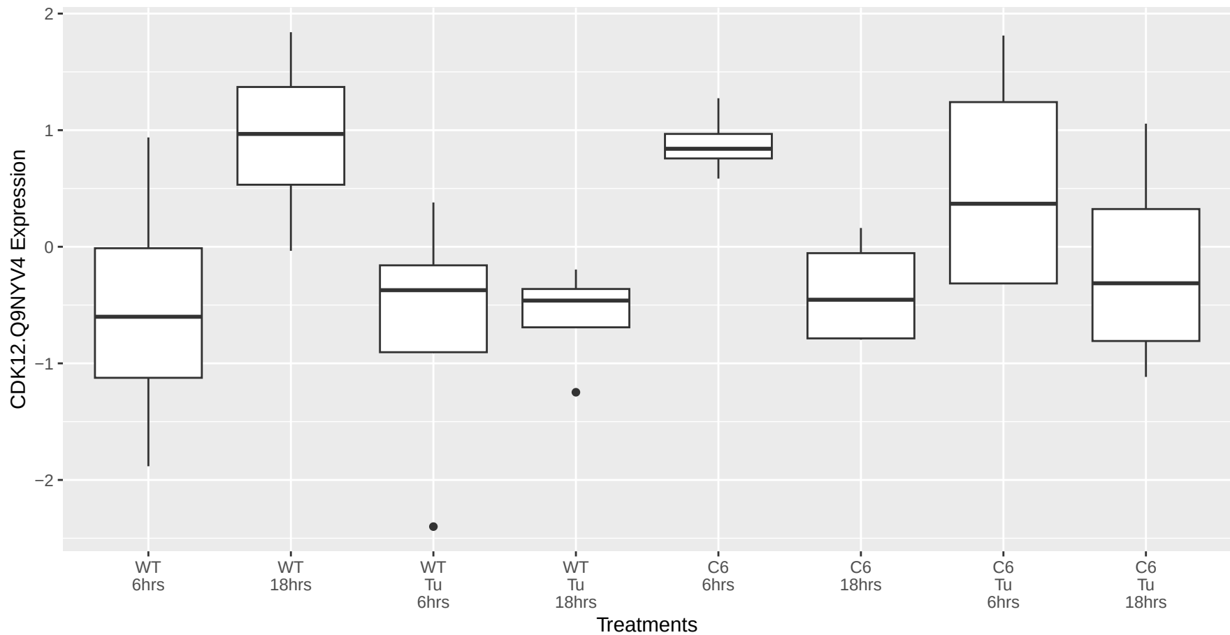
CDK12.Q9NYV4 occurs in the black module
