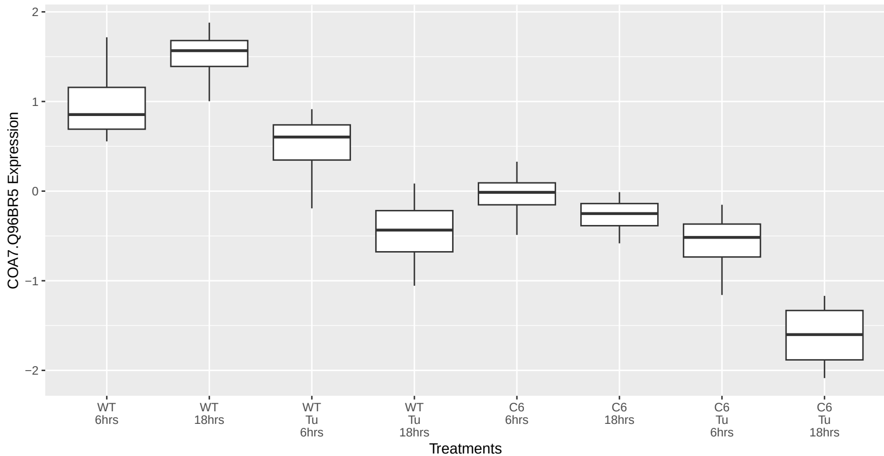
COA7.Q96BR5 occurs in the blue module
