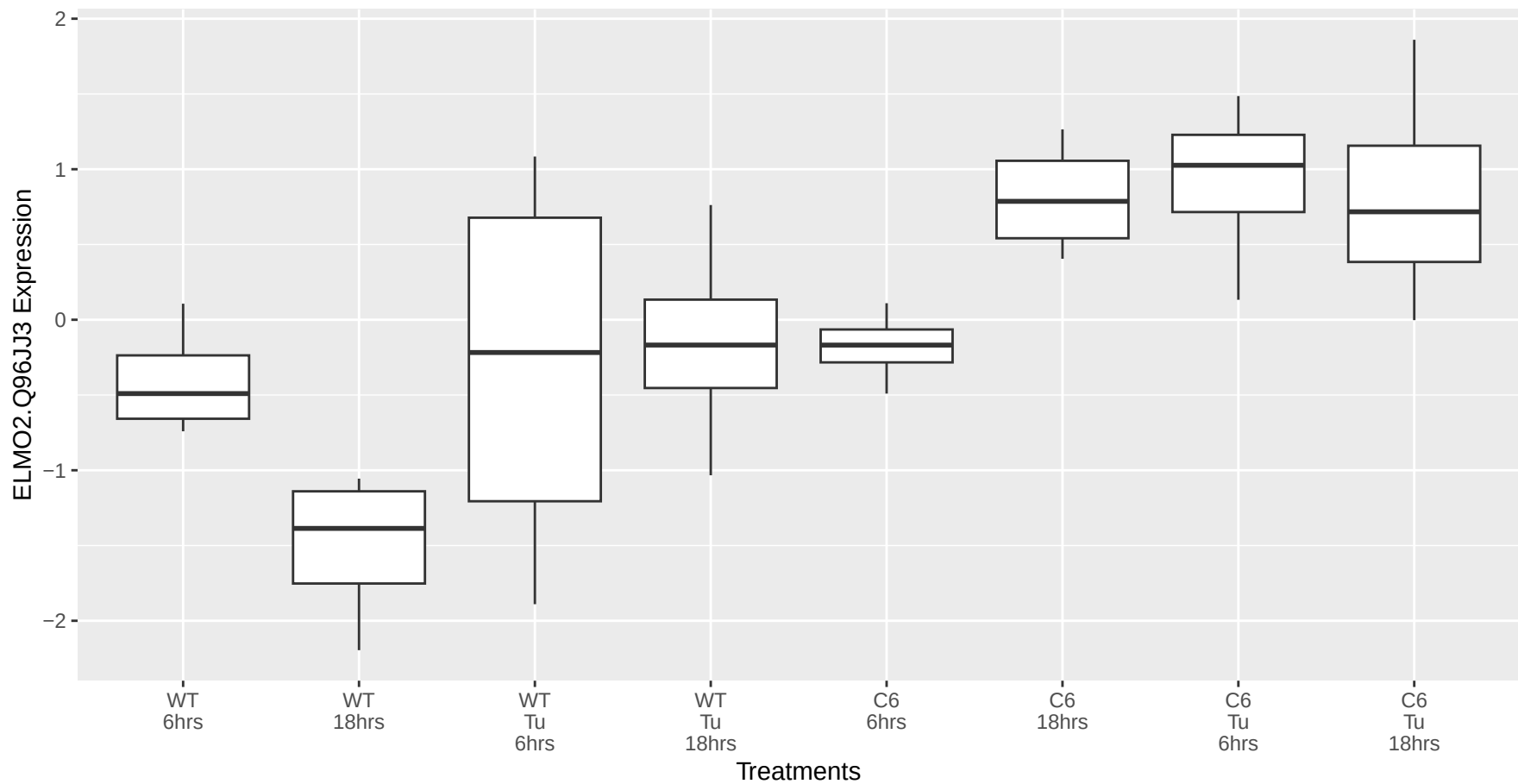
ELMO2.Q96JJ3 occurs in the blue module
