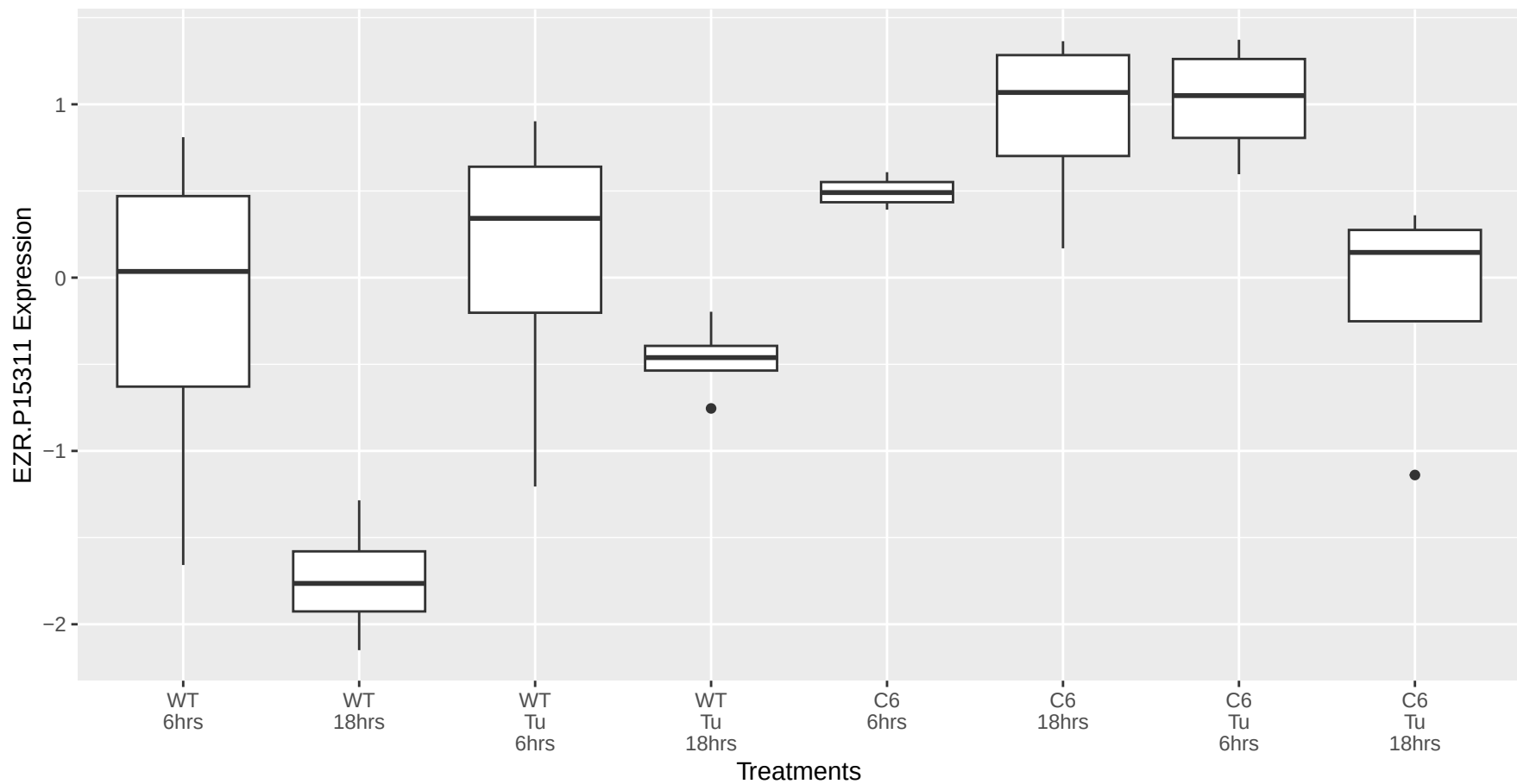
EZR.P15311 occurs in the brown module
