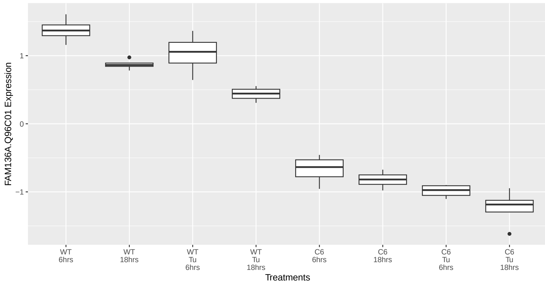
FAM136A.Q96C01 occurs in the magenta module
